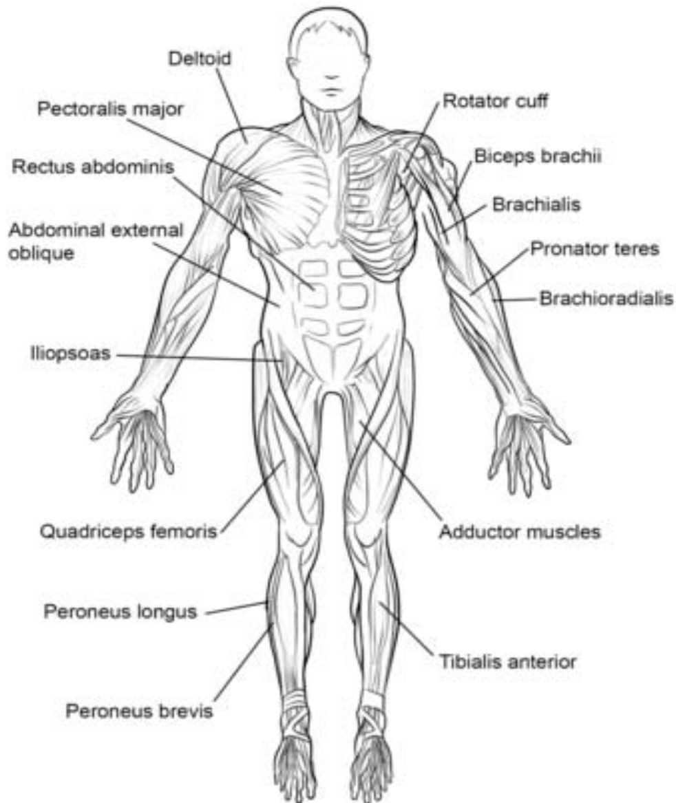
Human Muscles
